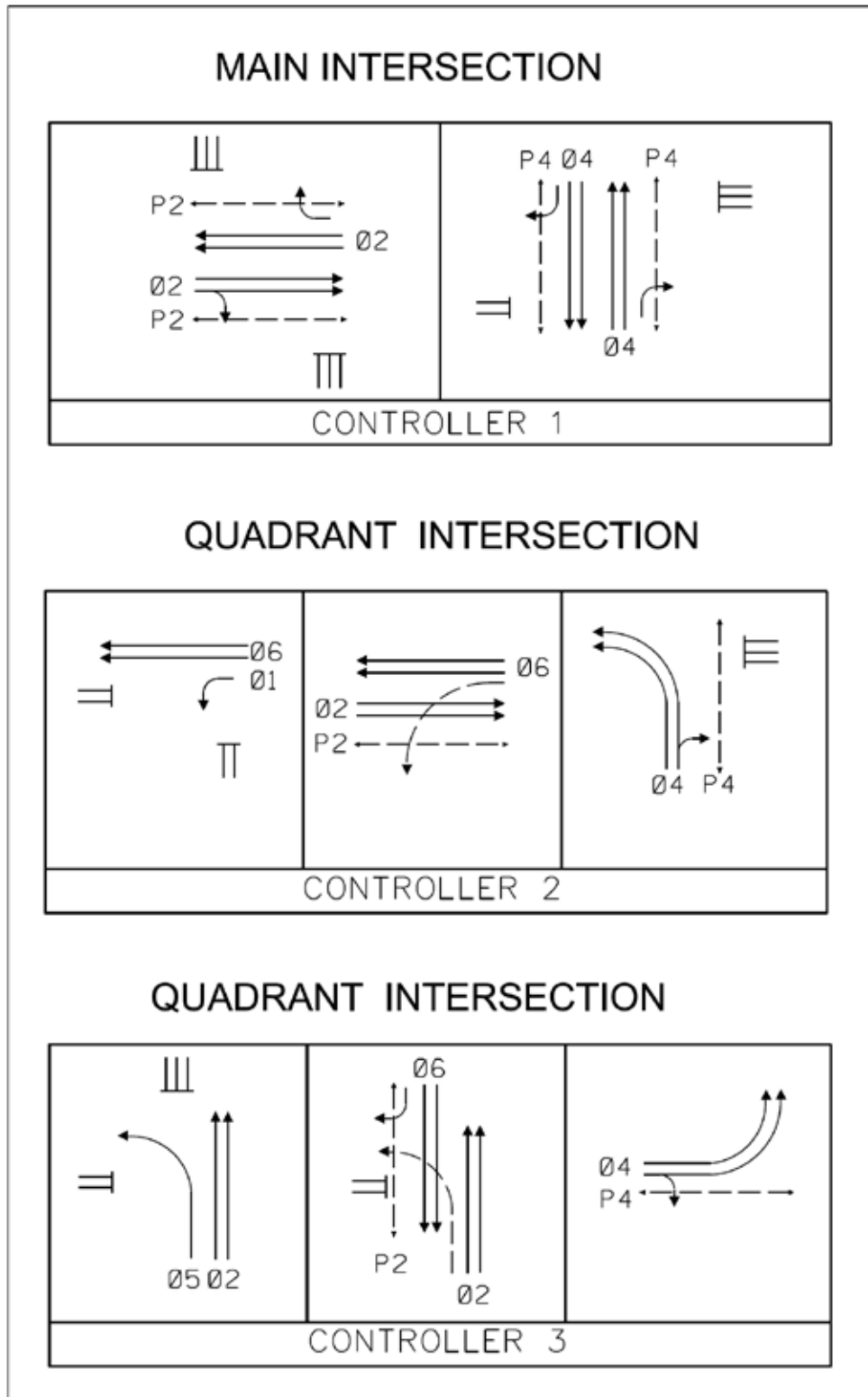
Figure 131. Illustration. QR intersection signal phasing scheme for separate controllers.
