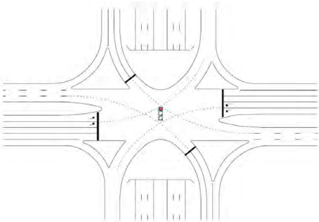
Figure 198. Illustration. SPUI configuration. (92)
