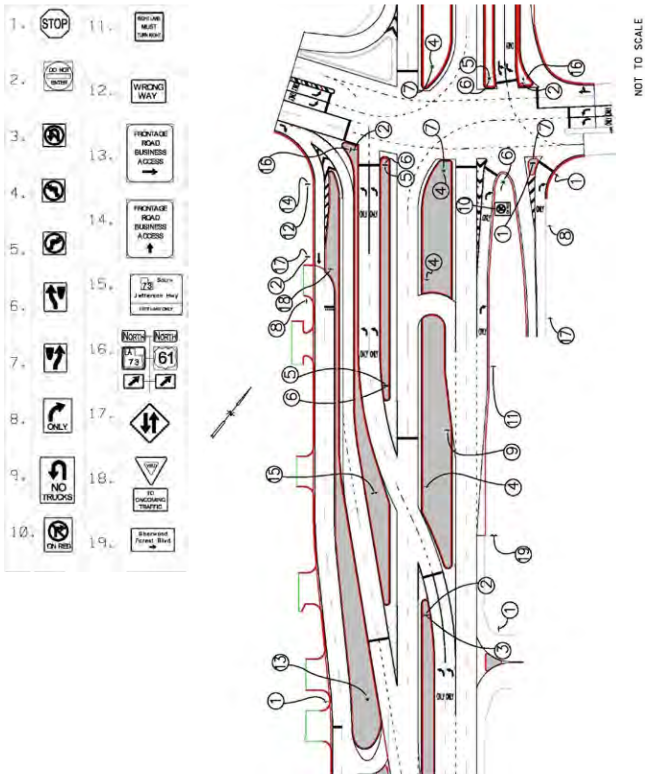
Figure 32. Illustration. Ground-mounted signing and marking as used at the DLT intersection in Baton Rouge, LA.
