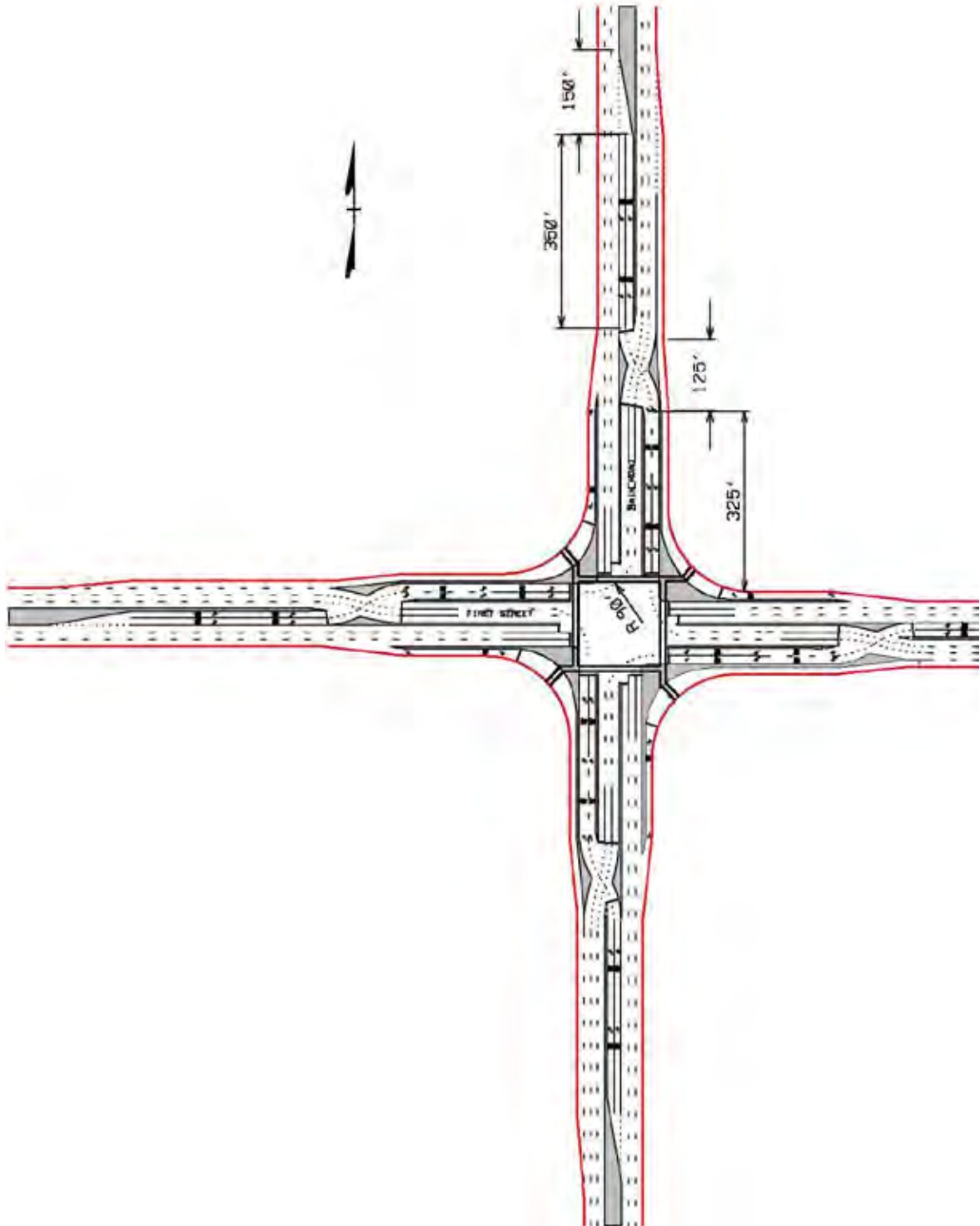
Figure 8. Illustration. Typical full DLT intersection plan view with DLTs on all approaches.
