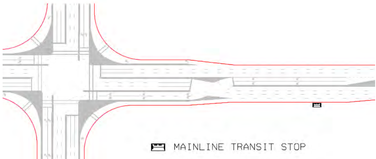
Figure 38. Illustration. Possible transit stop location in a DLT intersection.
