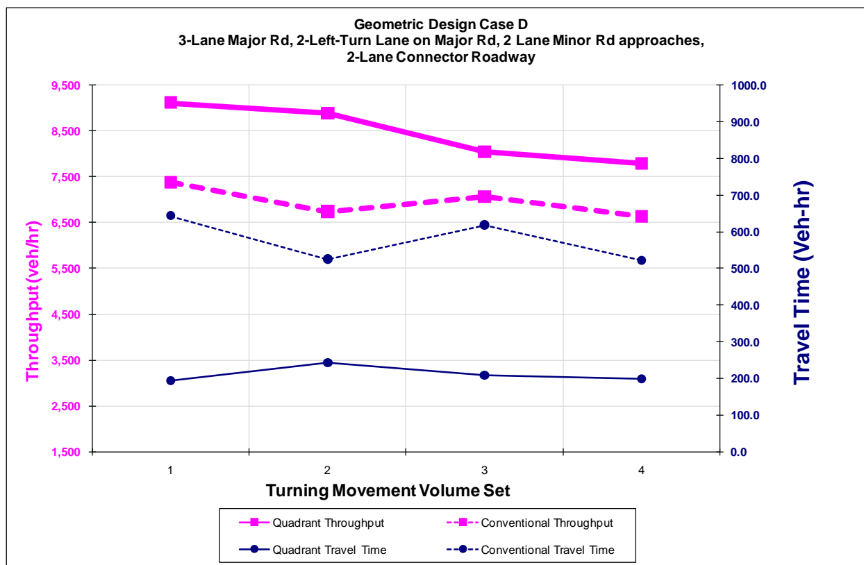
Figure 139. Graph. Throughput and travel time comparisons for geometric design case D.
