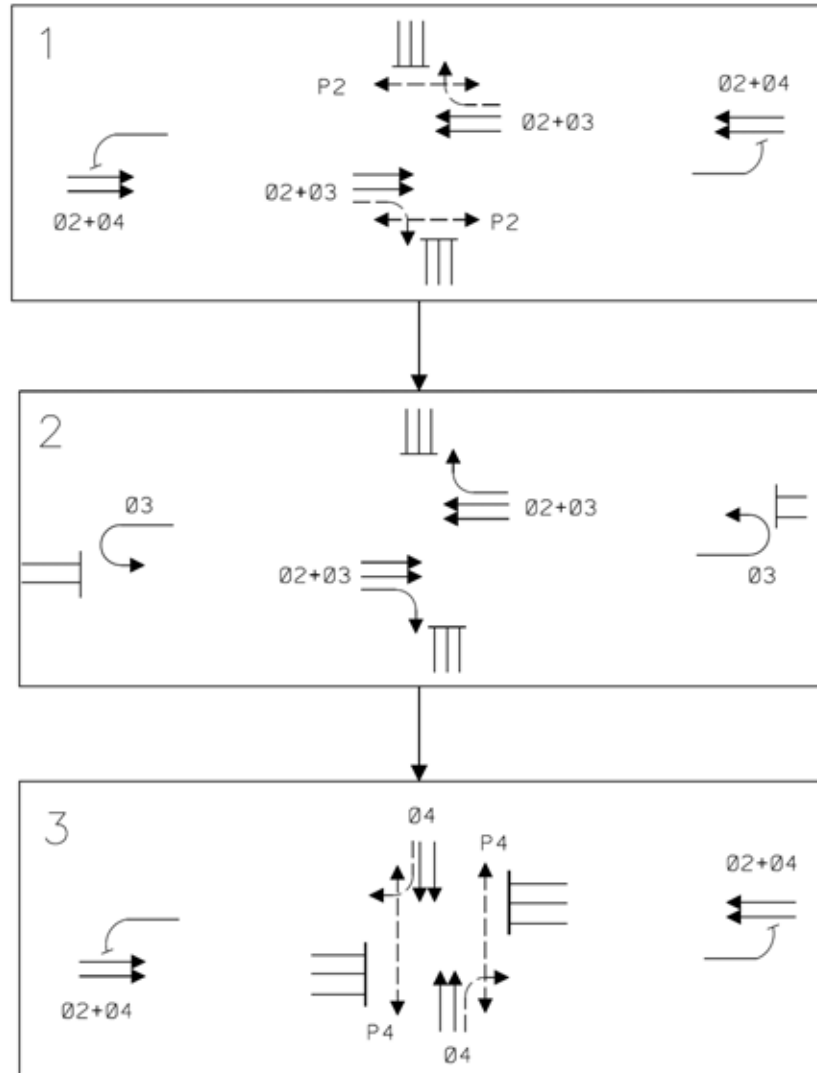
Figure 63. Illustration. Example MUT intersection phasing plan with overlaps.
