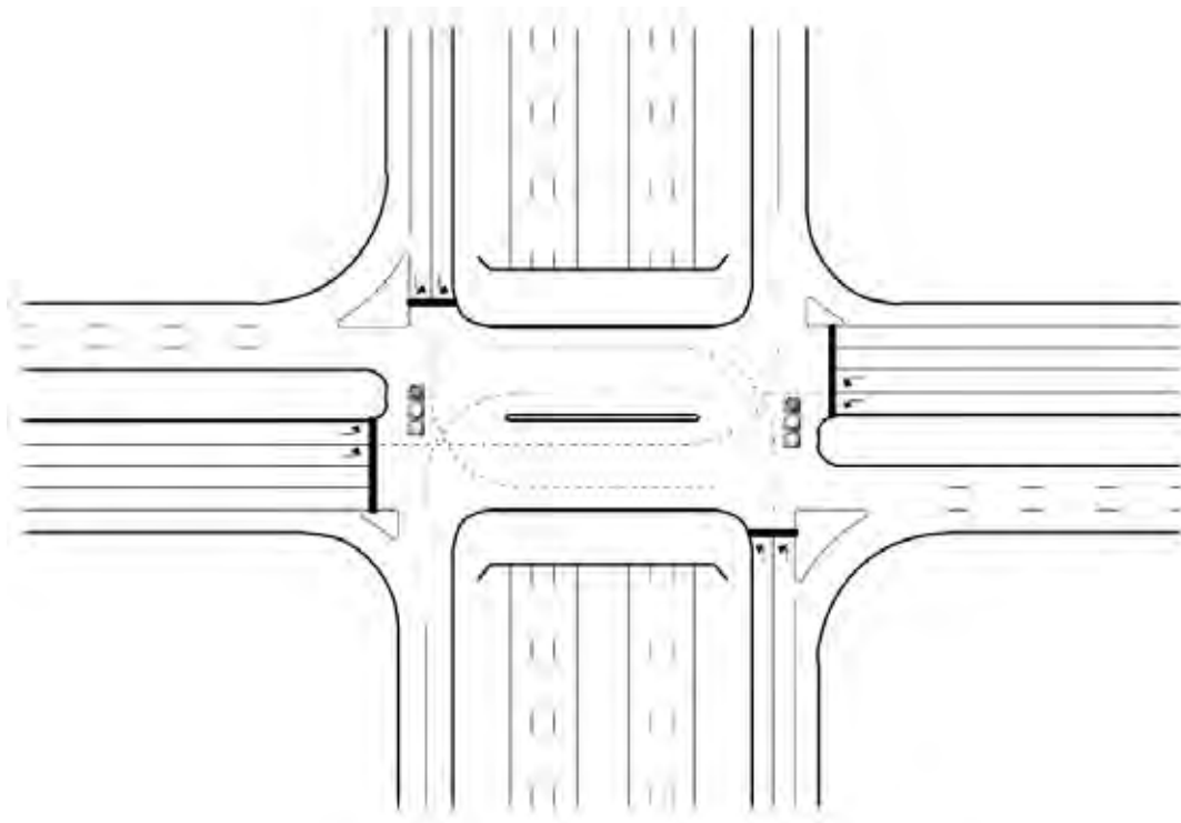
Figure 197. Illustration. TUDI configuration. (92)
