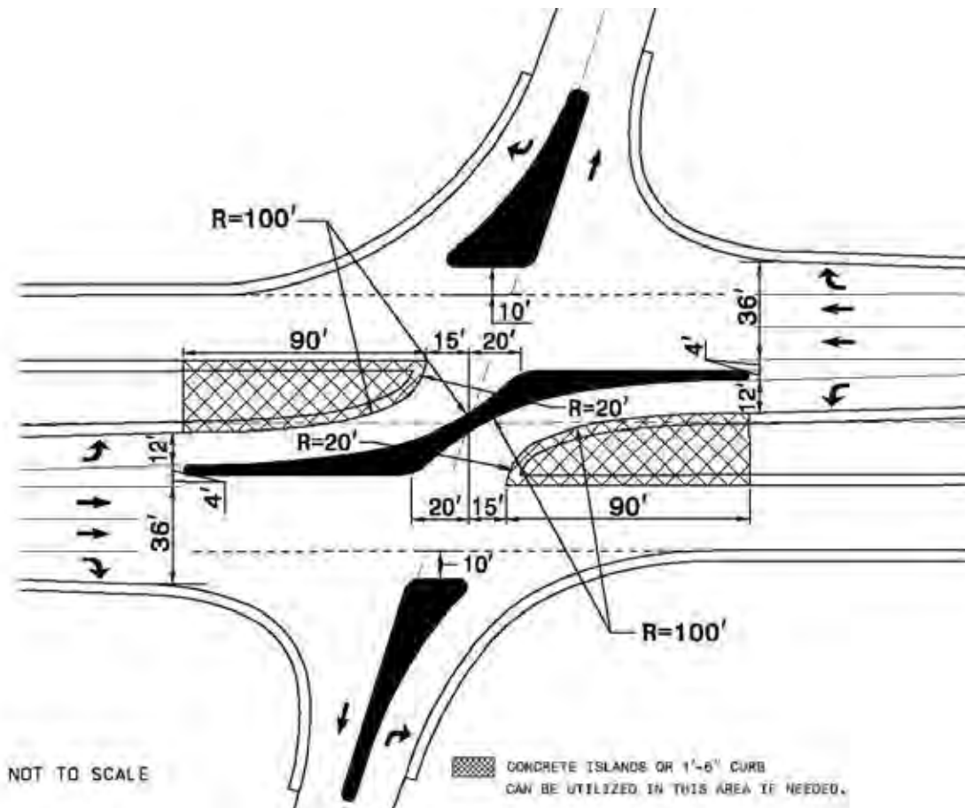
Figure 96. Illustration. NCDOT RCUT intersection left-turn crossover design recommendation. (57)
