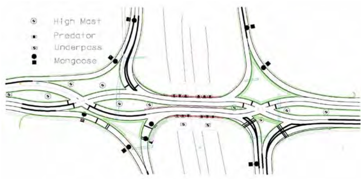
Figure 183. Illustration. Lighting plan being implemented at a DCD interchange in Kansas City, MO.
