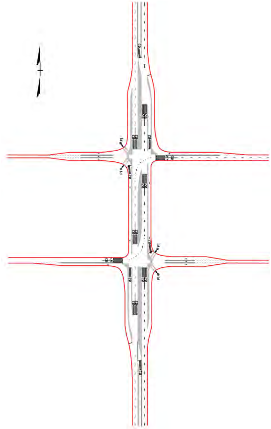
Figure 191. Illustration. Detector locations for a DLT interchange for signal phasing.
