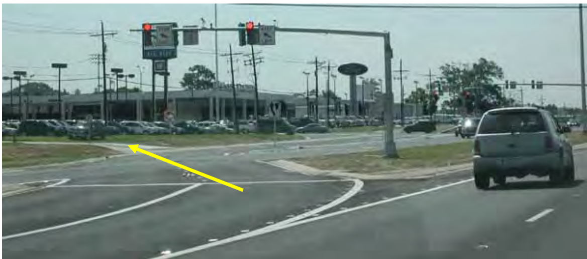
Figure 15. Photo. Right-in, right-out driveway accessible via the right-turn merge lane/frontage road at the DLT intersection in Baton Rouge, LA.
