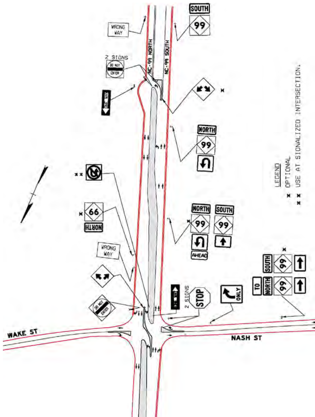
Figure 109. Illustration. RCUT intersection signing guidance from the NCDOT practice. (58)
