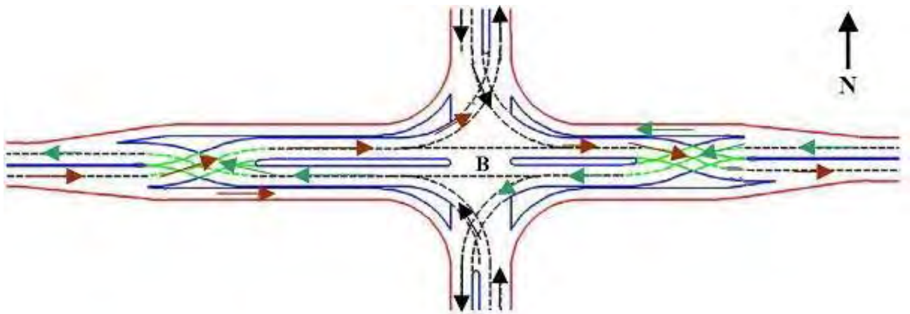
Figure 147. Illustration. Typical synchronized split-phase intersection movements. (76)
