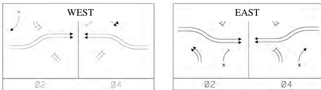
Figure 165. Illustration. Signal phasing for a DCD interchange operating under separate controllers.
