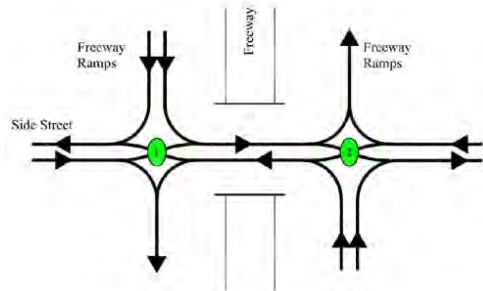
Figure 163. Illustration. Typical DCD interchange signal locations.
