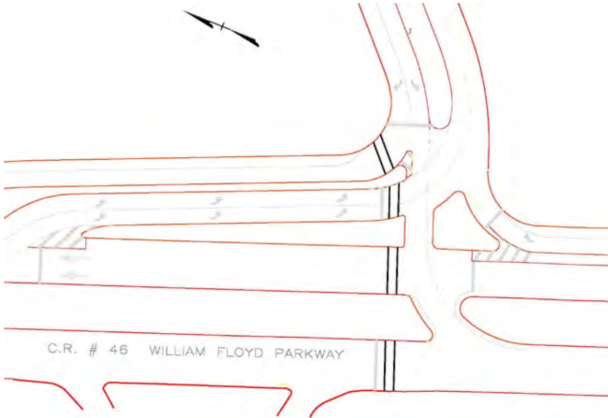
Figure 37. Illustration. Pedestrian crosswalks as implemented at DLT intersection at the entrance of Dowling NAT Center, Shirley, NY.
