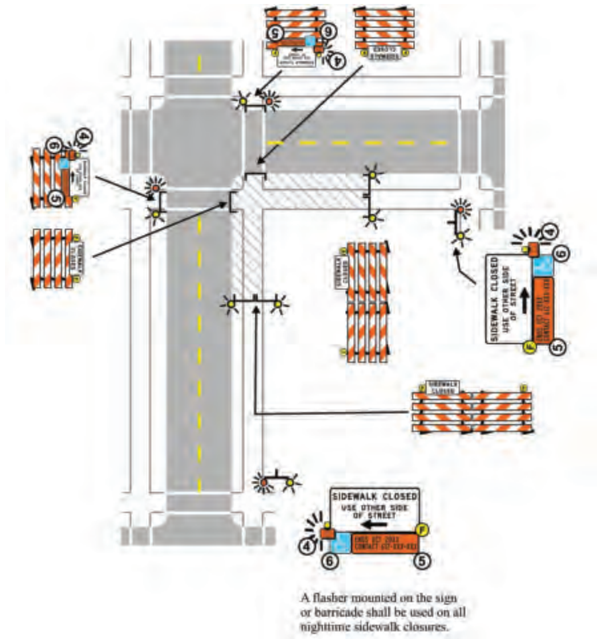
Figure 8. Layout 84B: Crosswalk Closures and Pedestrian Detours
