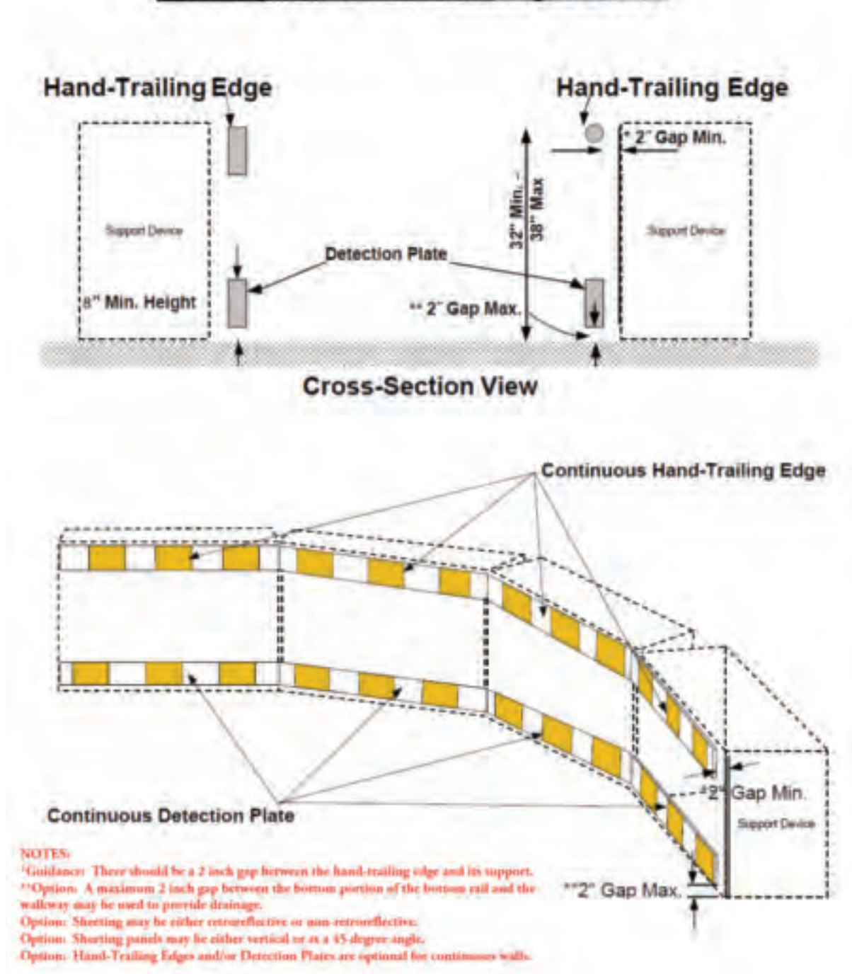
Figure 6F-XX Pedestrian Channelizing Device
