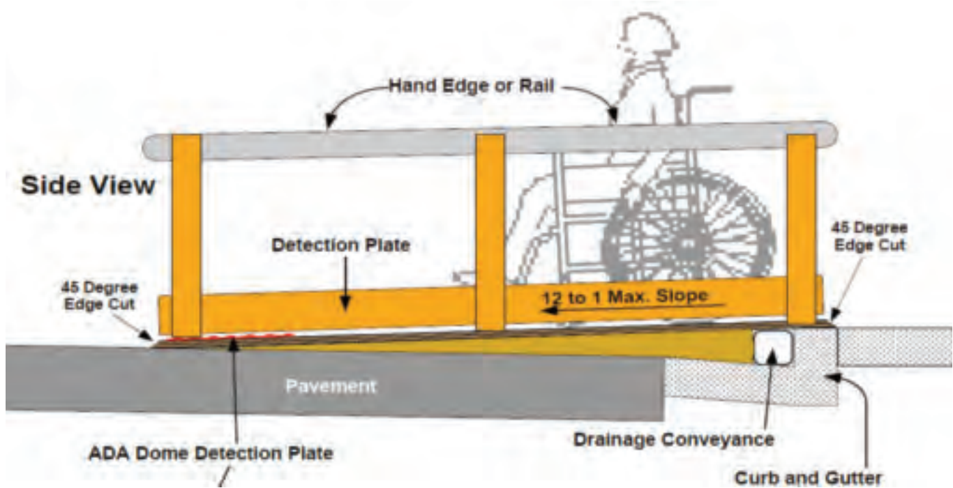
Figure 21. Pedestrian/ADA Detour Path – Temporary Ramp into the Roadway
