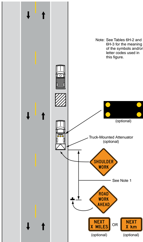
Typical Application 4
