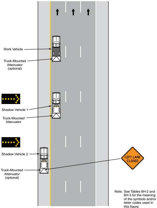
Typical Application 35
